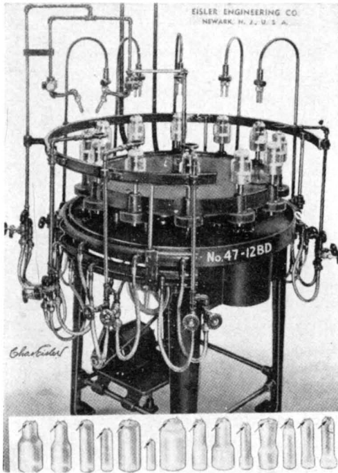
The Eisler bulb-piercing machine. (Patent No. 2,414,587.)
